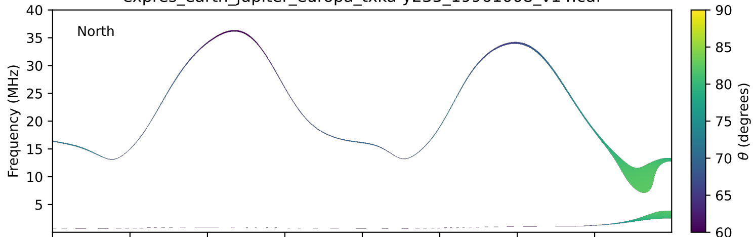
expres_earth_jupiter_europa_txka-y235_19961008_v14.cdf
