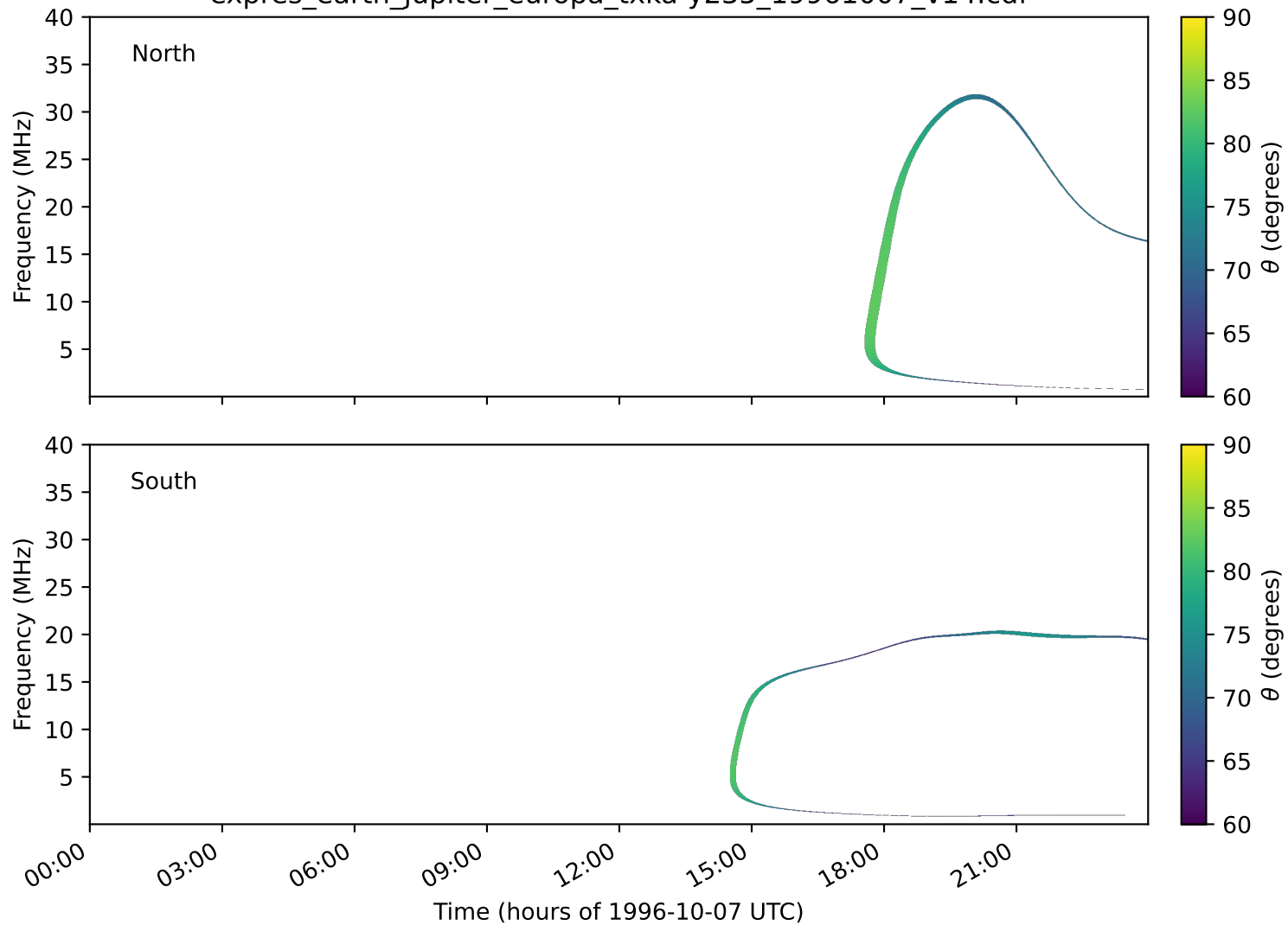
expres_earth_jupiter_europa_txka-y235_19961007_v14.cdf
