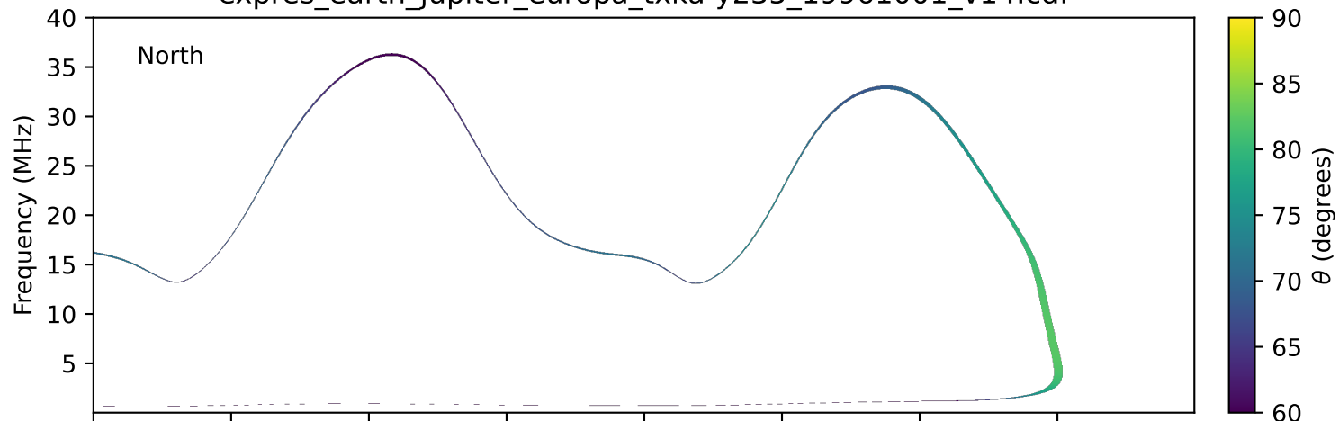
expres_earth_jupiter_europa_txka-y235_19961001_v14.cdf
