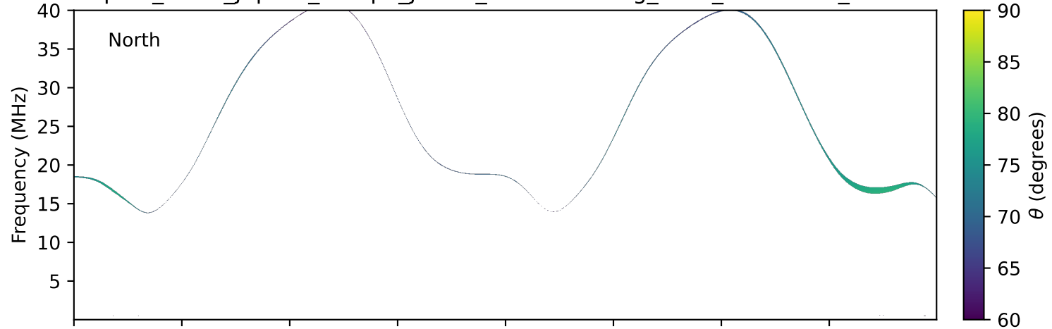
expres_earth_jupiter_europa_jrm33_lossc-wid1deg_3kev_19961008_v11.cdf
