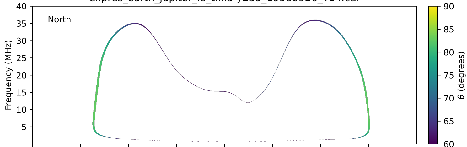
expres_earth_jupiter_io_txka-y235_19960926_v14.cdf
