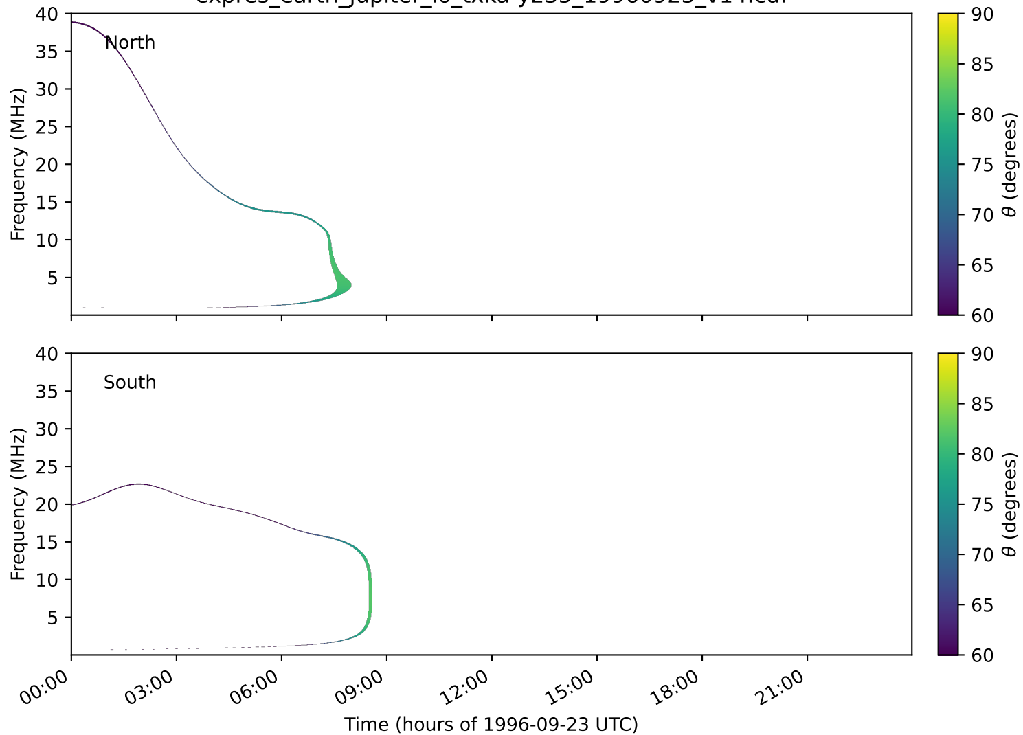
expres_earth_jupiter_io_txka-y235_19960923_v14.cdf
