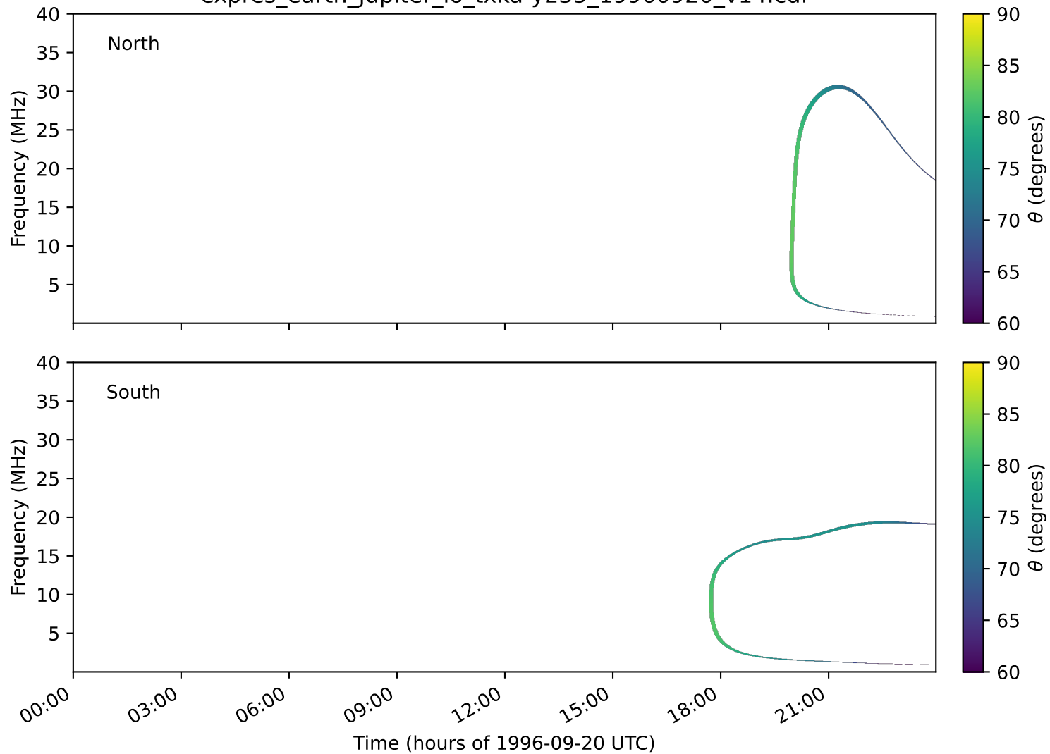
expres_earth_jupiter_io_txka-y235_19960920_v14.cdf
