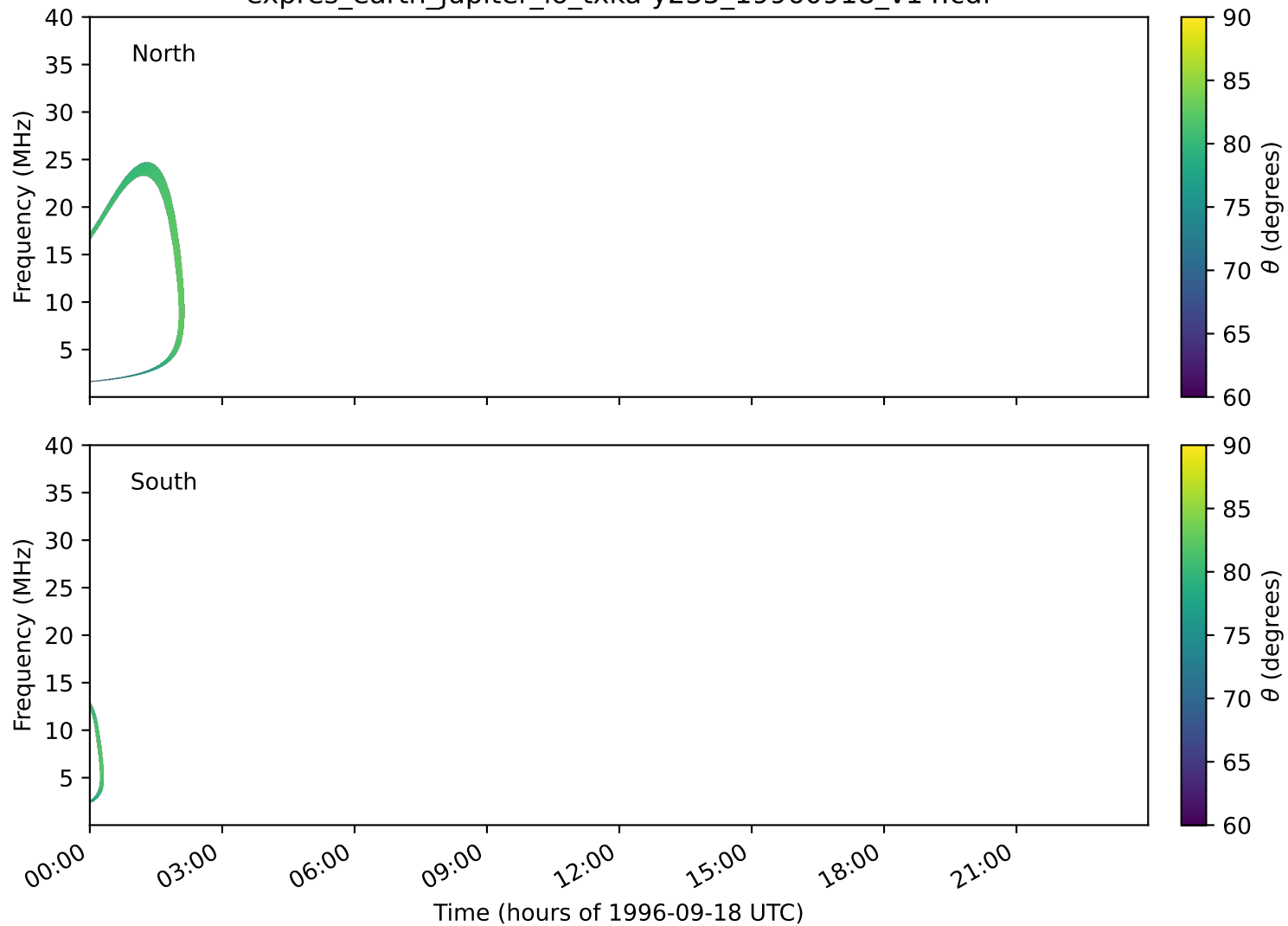
expres_earth_jupiter_io_txka-y235_19960918_v14.cdf
