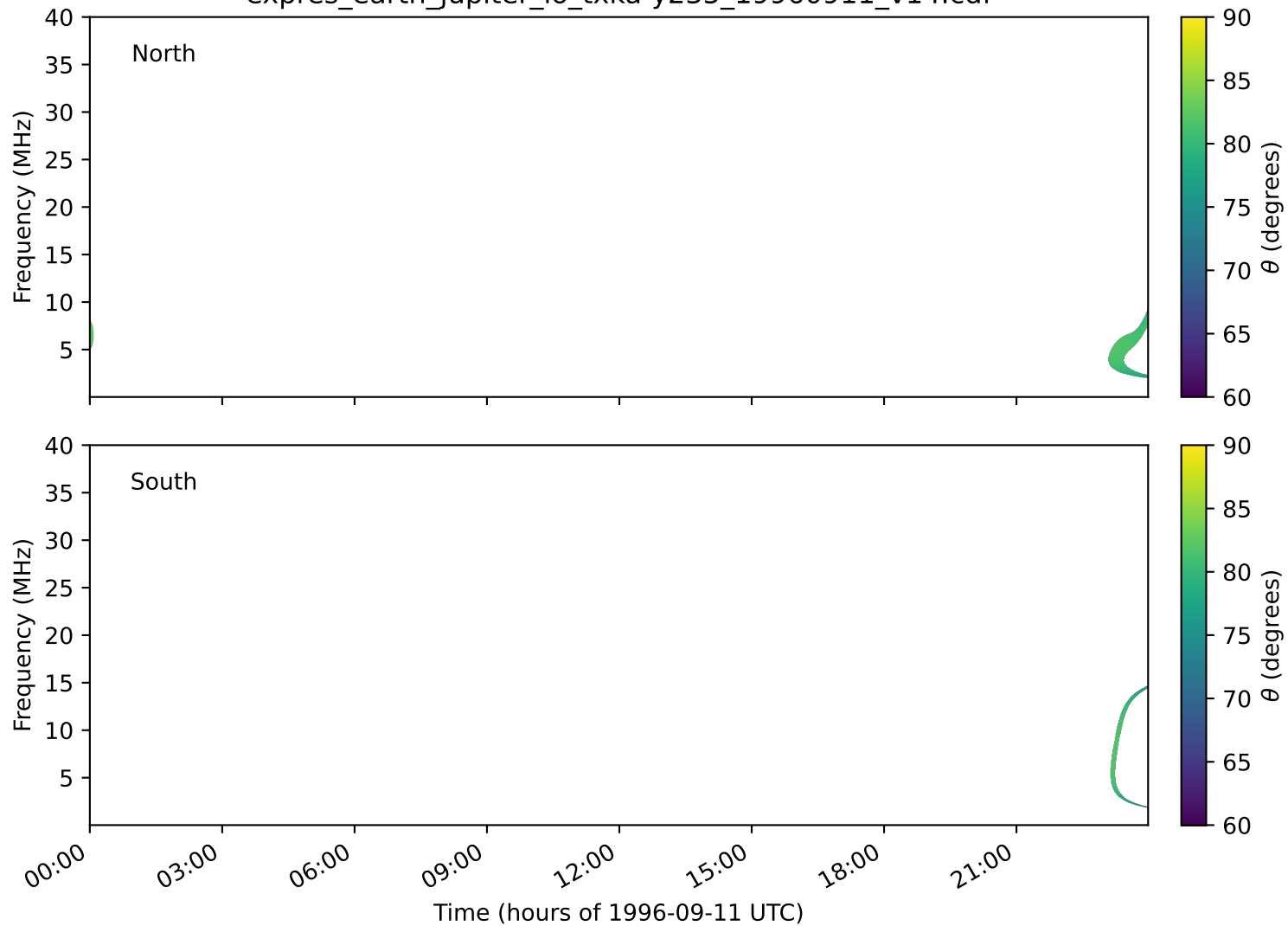
expres_earth_jupiter_io_txka-y235_19960911_v14.cdf
