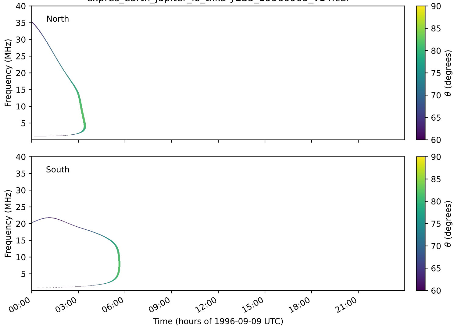
expres_earth_jupiter_io_txka-y235_19960909_v14.cdf
