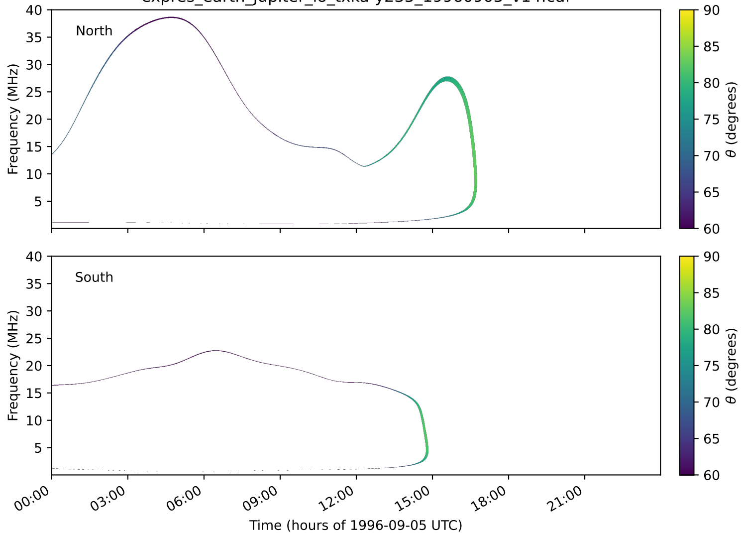
expres_earth_jupiter_io_txka-y235_19960905_v14.cdf
