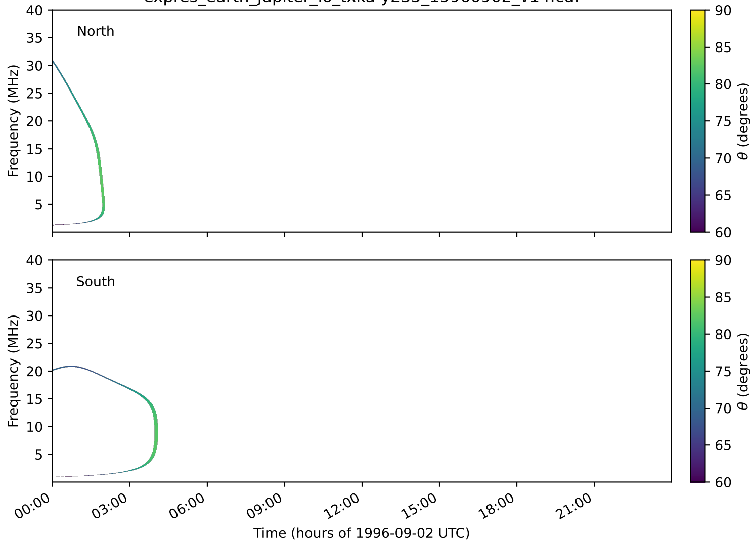
expres_earth_jupiter_io_txka-y235_19960902_v14.cdf
