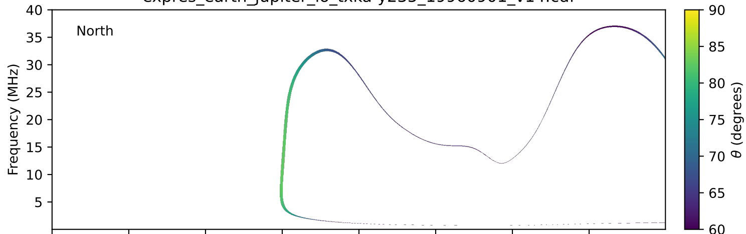
expres_earth_jupiter_io_txka-y235_19960901_v14.cdf
