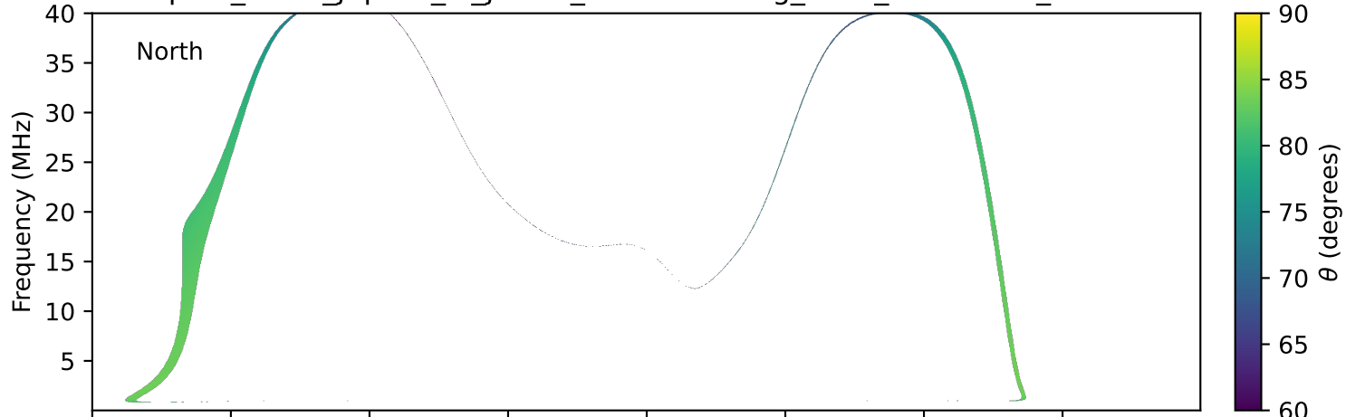
expres_earth_jupiter_io_jrm33_lossc-wid1deg_3kev_19960919_v11.cdf
