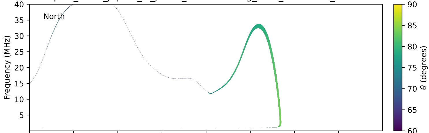
expres_earth_jupiter_io_jrm33_lossc-wid1deg_3kev_19960905_v11.cdf
