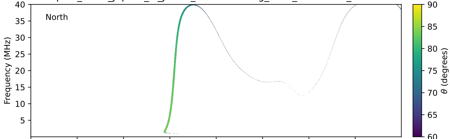
expres_earth_jupiter_io_jrm33_lossc-wid1deg_3kev_19960901_v11.cdf
