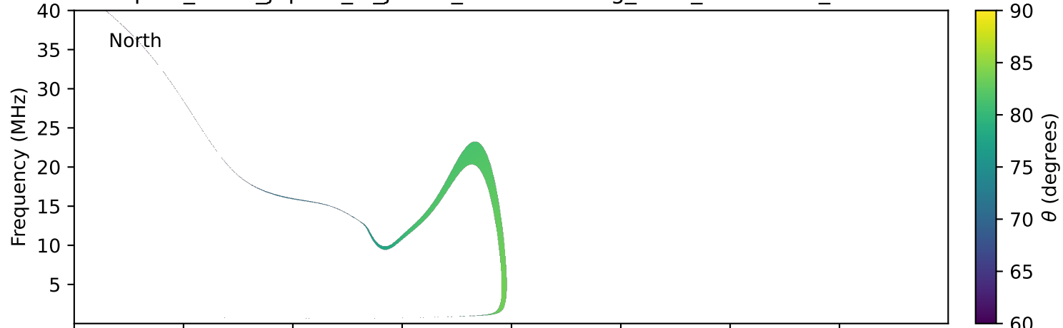
expres_earth_jupiter_io_jrm09_lossc-wid1deg_3kev_19960930_v11.cdf
