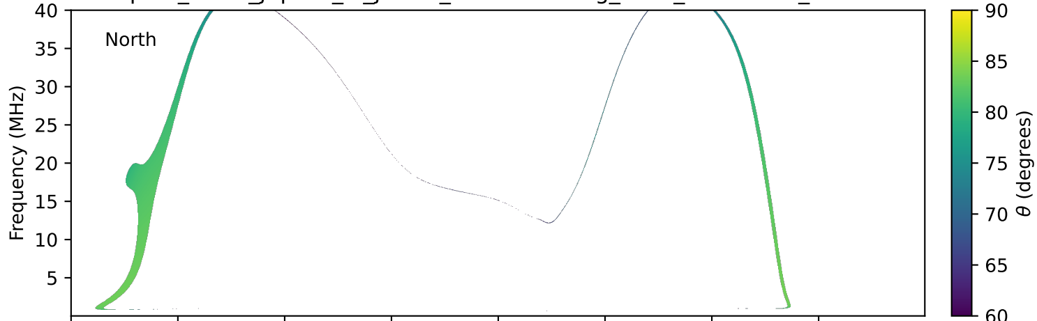
expres_earth_jupiter_io_jrm09_lossc-wid1deg_3kev_19960919_v11.cdf
