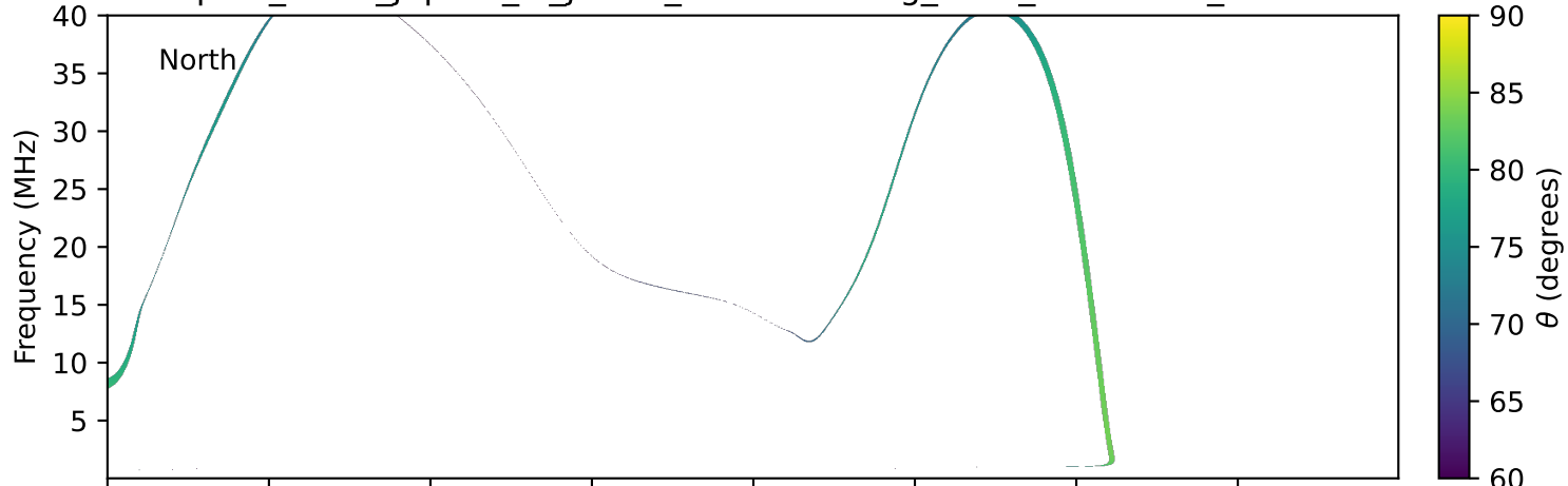
expres_earth_jupiter_io_jrm09_lossc-wid1deg_3kev_19960912_v11.cdf
