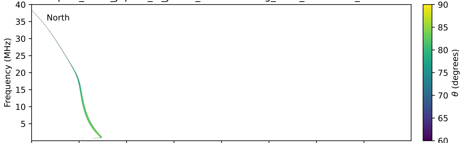
expres_earth_jupiter_io_jrm09_lossc-wid1deg_3kev_19960909_v11.cdf
