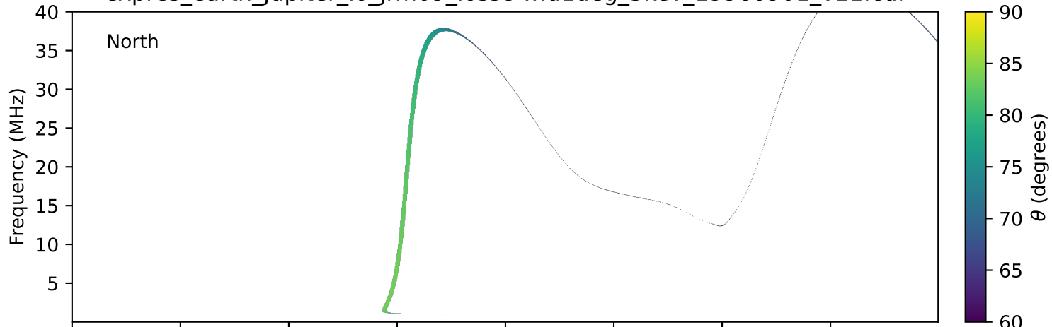
expres_earth_jupiter_io_jrm09_lossc-wid1deg_3kev_19960901_v11.cdf
