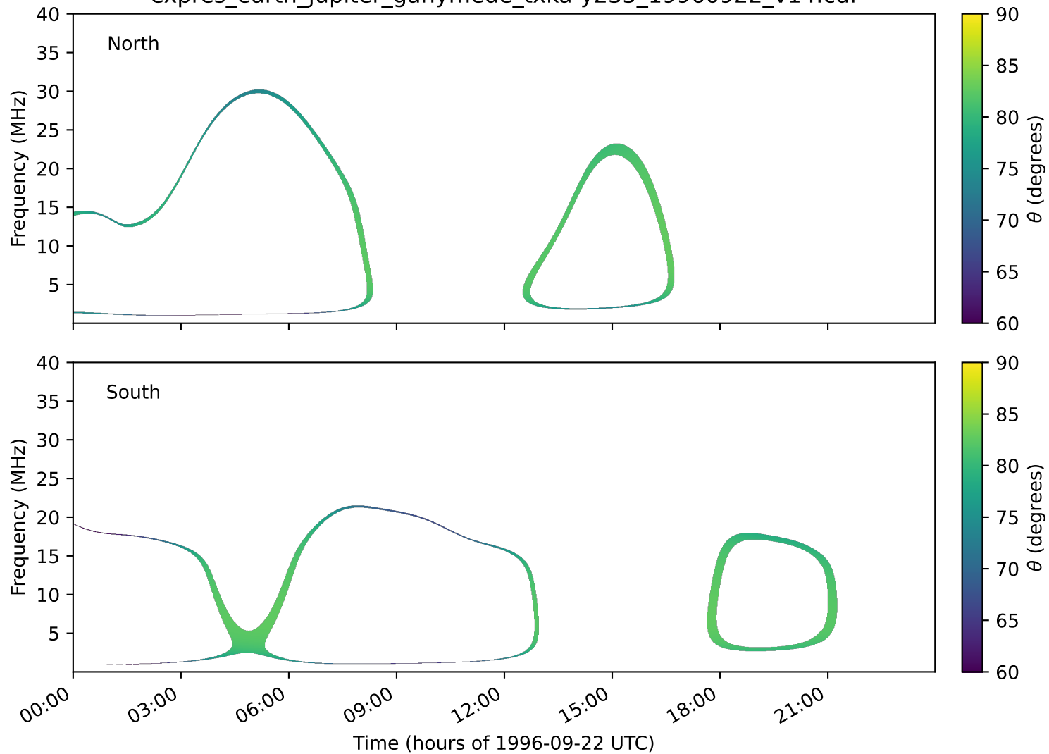
expres_earth_jupiter_ganymede_txka-y235_19960922_v14.cdf
