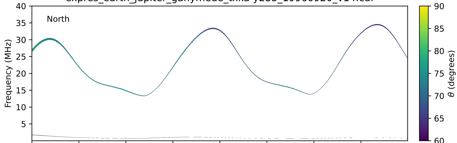
expres_earth_jupiter_ganymede_txka-y235_19960920_v14.cdf
