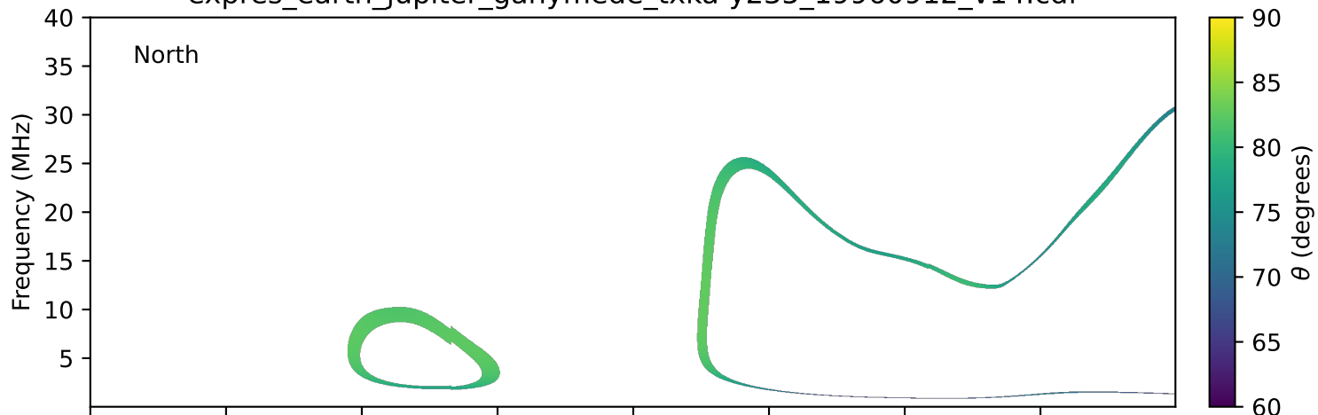
expres_earth_jupiter_ganymede_txka-y235_19960912_v14.cdf
