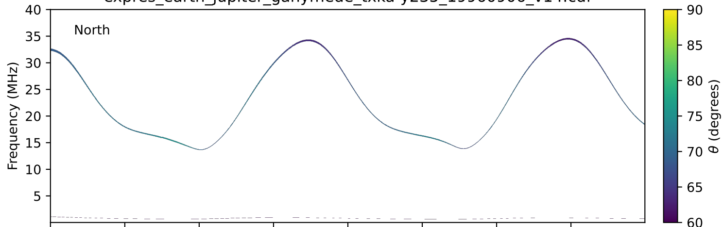
expres_earth_jupiter_ganymede_txka-y235_19960906_v14.cdf
