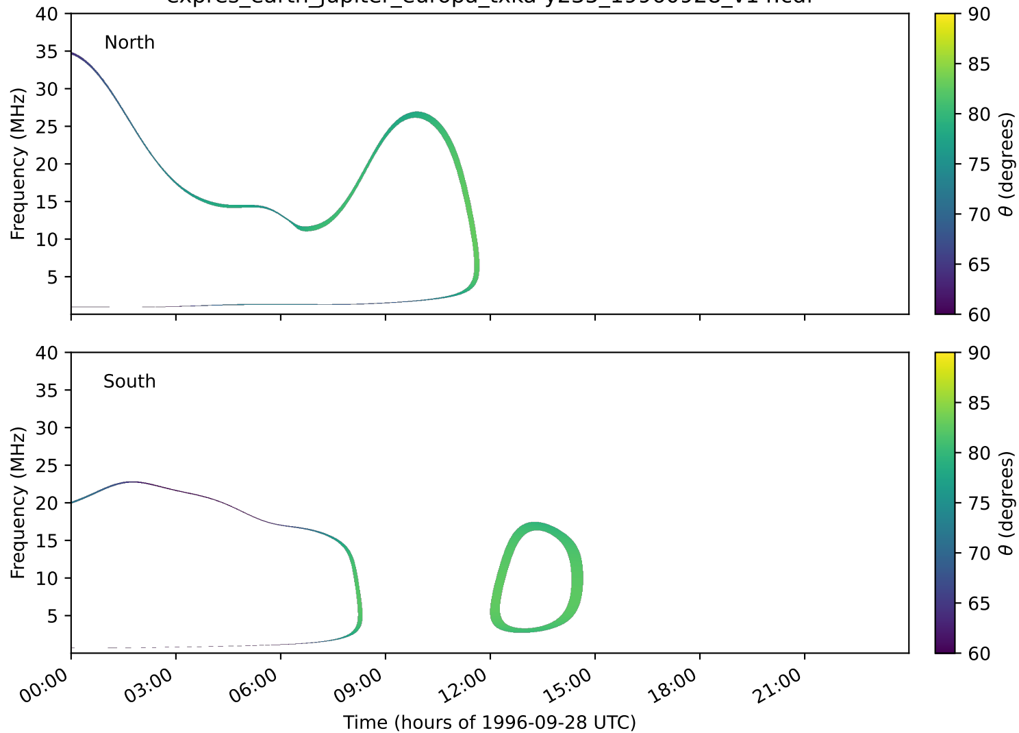
expres_earth_jupiter_europa_txka-y235_19960928_v14.cdf
