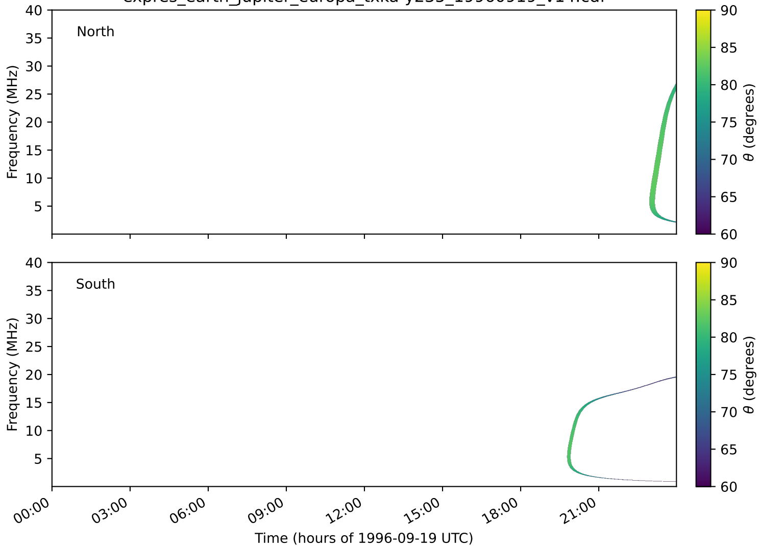
expres_earth_jupiter_europa_txka-y235_19960919_v14.cdf
