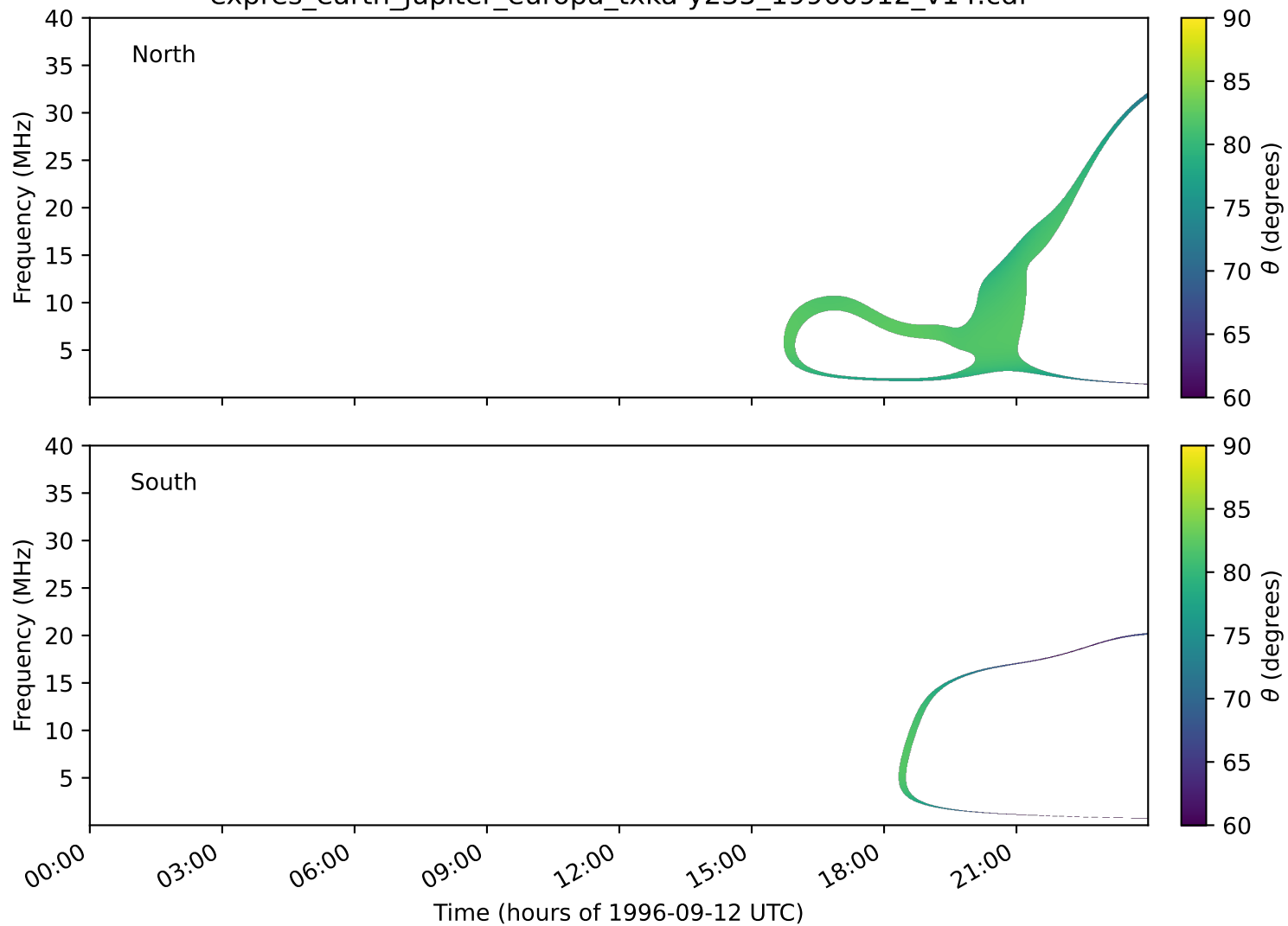
expres_earth_jupiter_europa_txka-y235_19960912_v14.cdf
