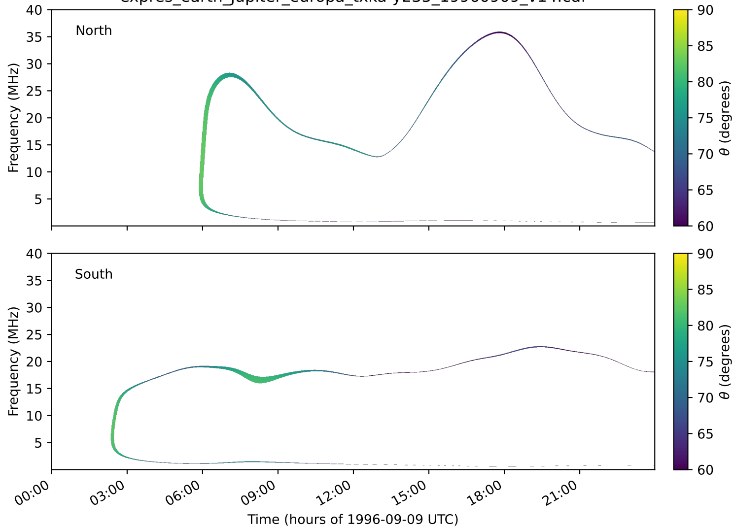
expres_earth_jupiter_europa_txka-y235_19960909_v14.cdf
