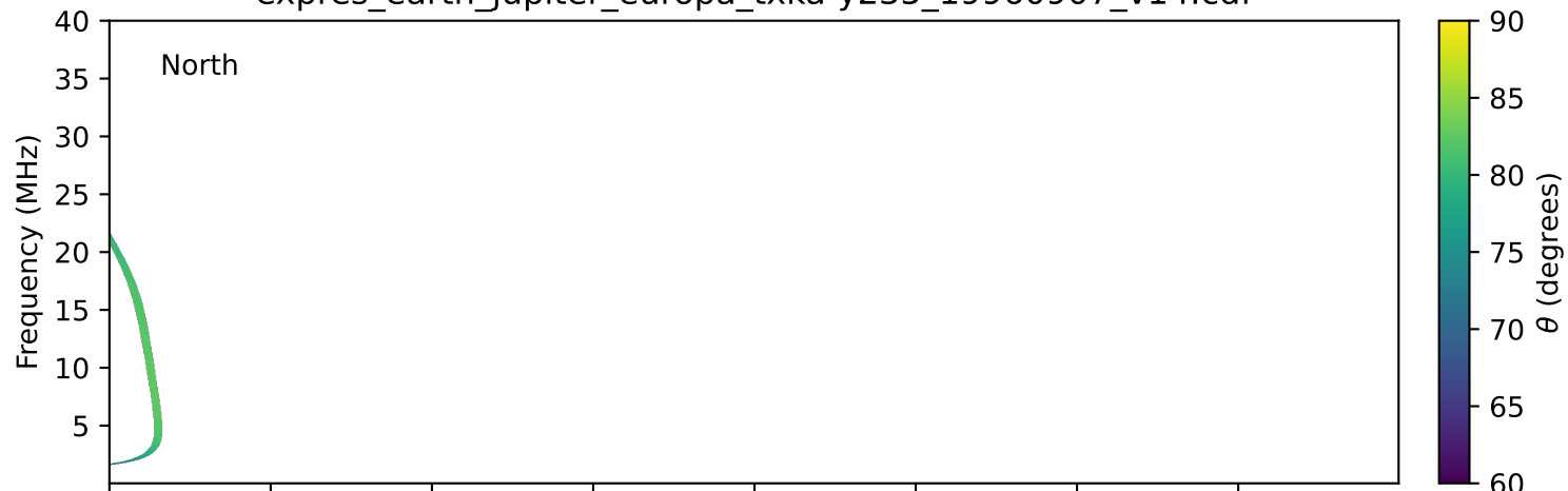
expres_earth_jupiter_europa_txka-y235_19960907_v14.cdf
