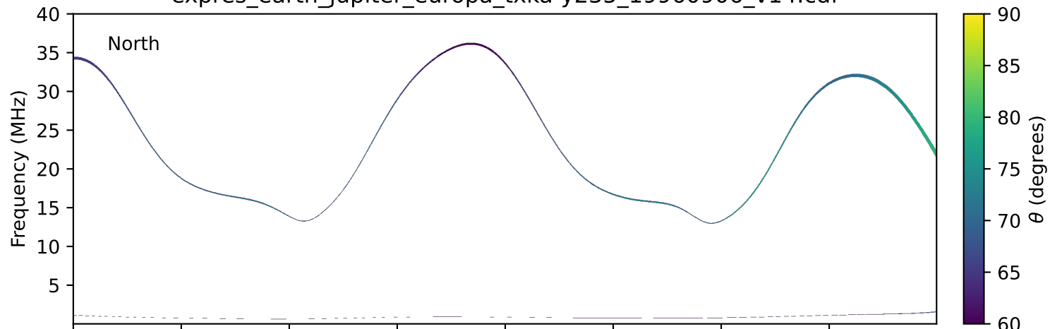
expres_earth_jupiter_europa_txka-y235_19960906_v14.cdf
