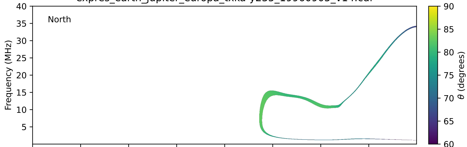
expres_earth_jupiter_europa_txka-y235_19960905_v14.cdf
