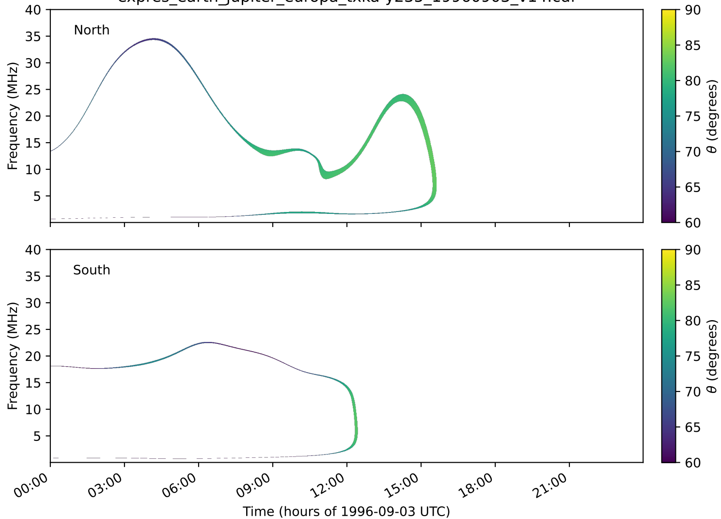
expres_earth_jupiter_europa_txka-y235_19960903_v14.cdf
