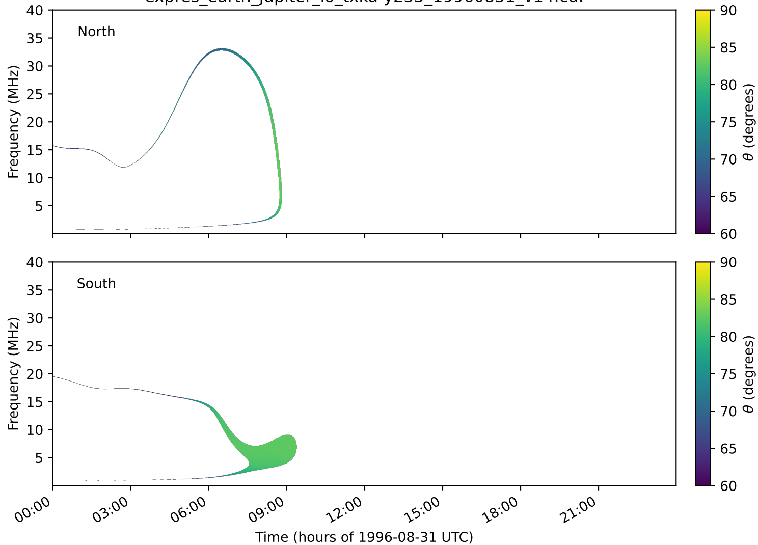
expres_earth_jupiter_io_txka-y235_19960831_v14.cdf
