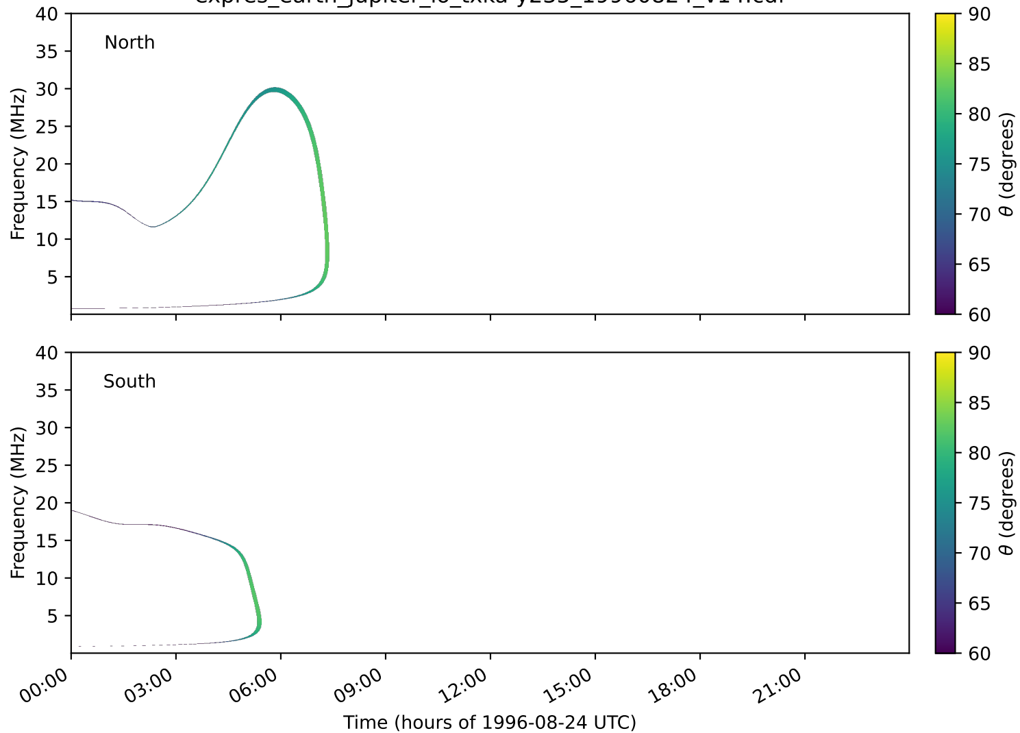
expres_earth_jupiter_io_txka-y235_19960824_v14.cdf
