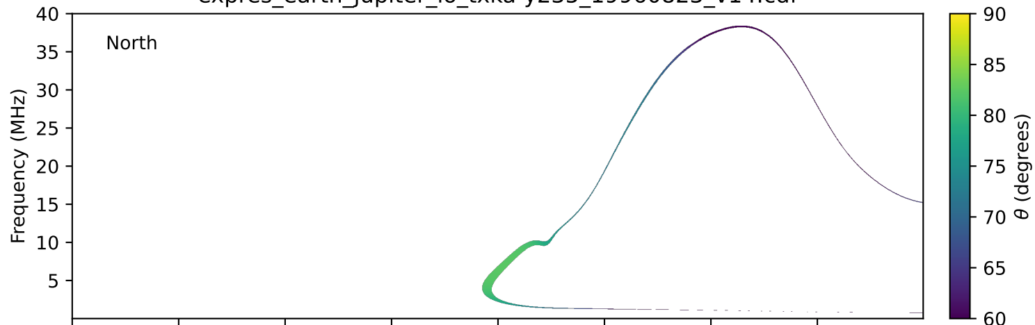
expres_earth_jupiter_io_txka-y235_19960823_v14.cdf
