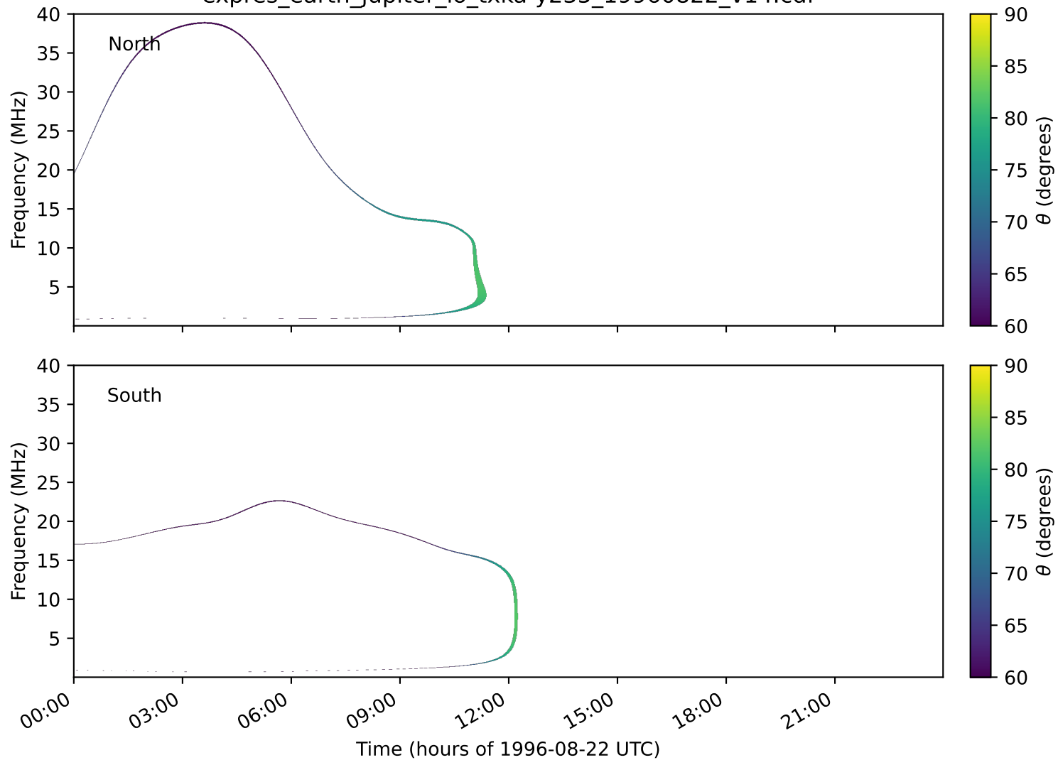
expres_earth_jupiter_io_txka-y235_19960822_v14.cdf
