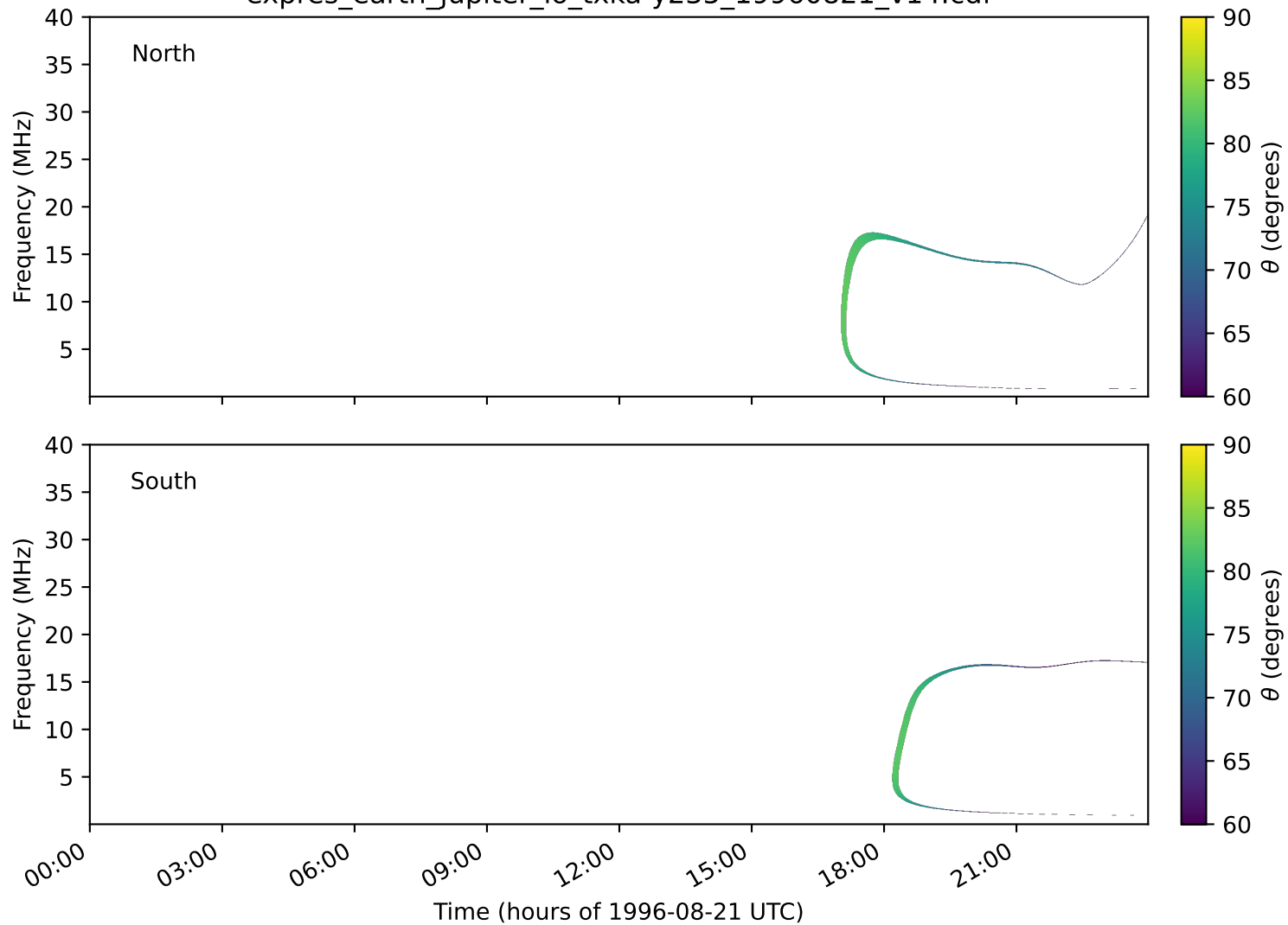
expres_earth_jupiter_io_txka-y235_19960821_v14.cdf
