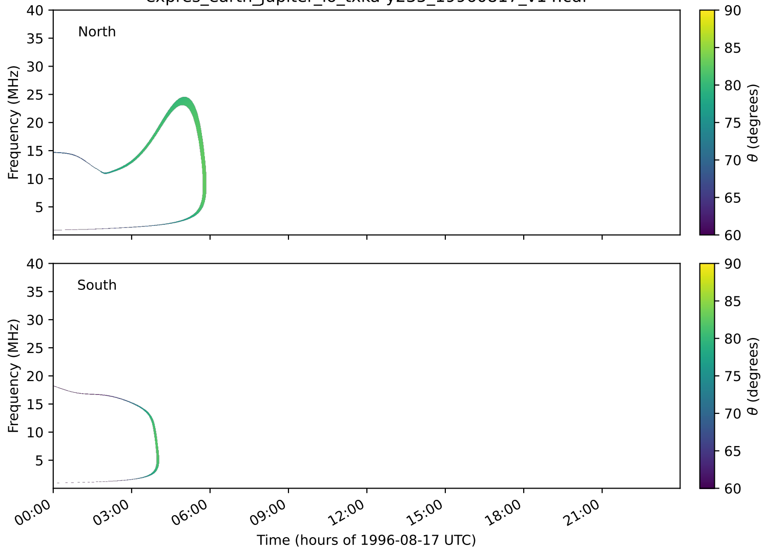
expres_earth_jupiter_io_txka-y235_19960817_v14.cdf
