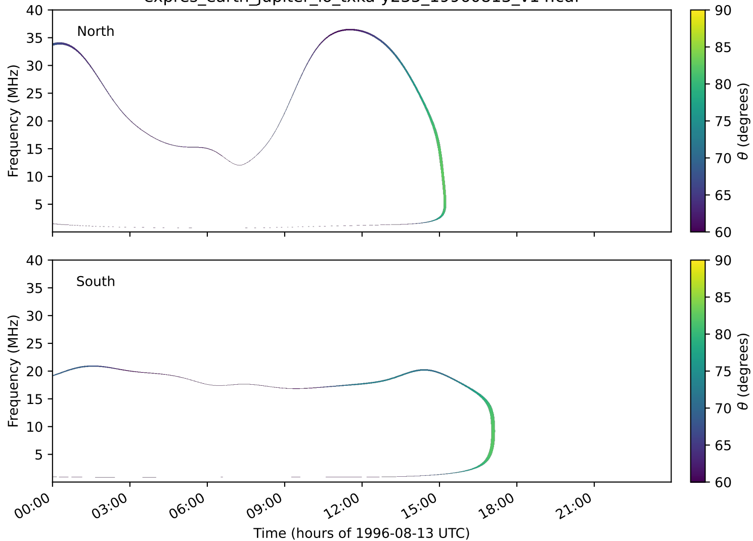
expres_earth_jupiter_io_txka-y235_19960813_v14.cdf
