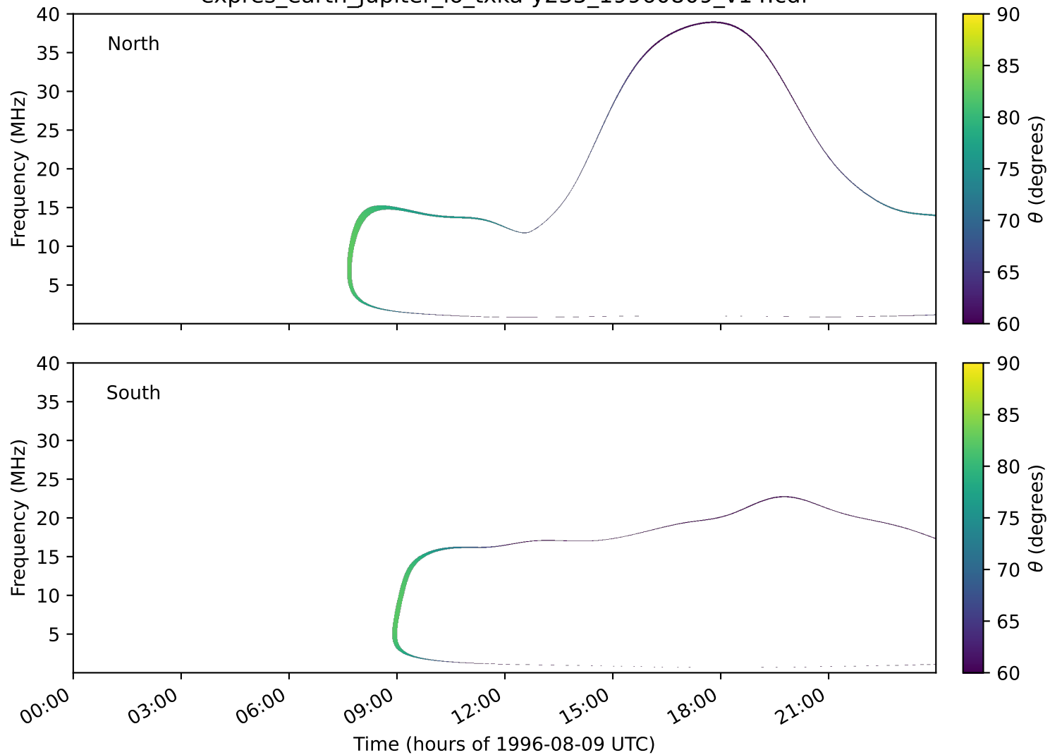
expres_earth_jupiter_io_txka-y235_19960809_v14.cdf
