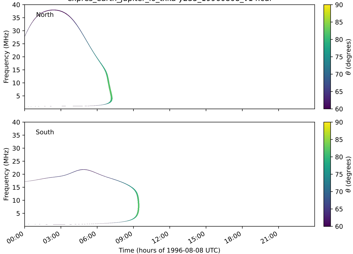
expres_earth_jupiter_io_txka-y235_19960808_v14.cdf
