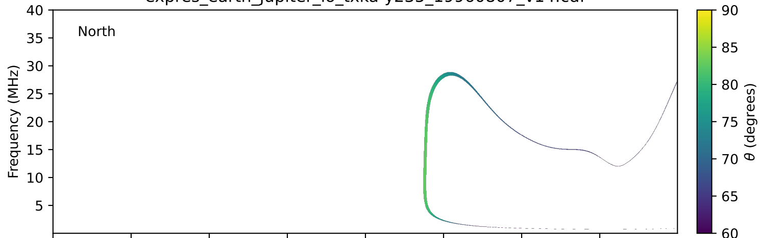
expres_earth_jupiter_io_txka-y235_19960807_v14.cdf
