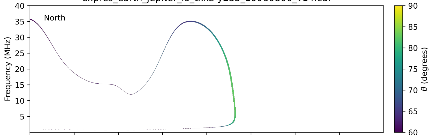
expres_earth_jupiter_io_txka-y235_19960806_v14.cdf
