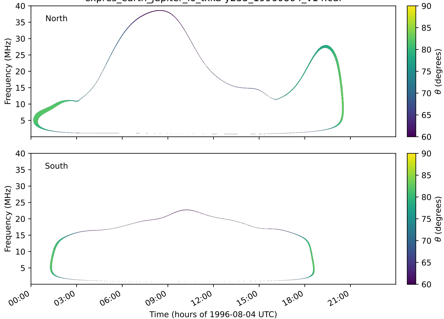
expres_earth_jupiter_io_txka-y235_19960804_v14.cdf
