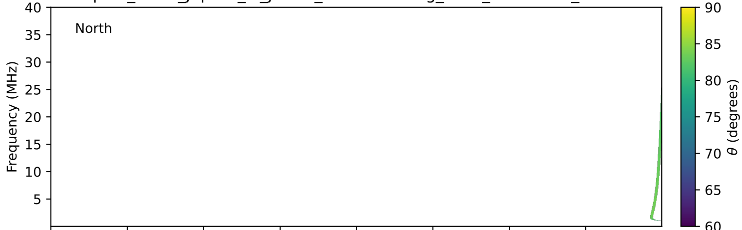
expres_earth_jupiter_io_jrm33_lossc-wid1deg_3kev_19960819_v11.cdf
