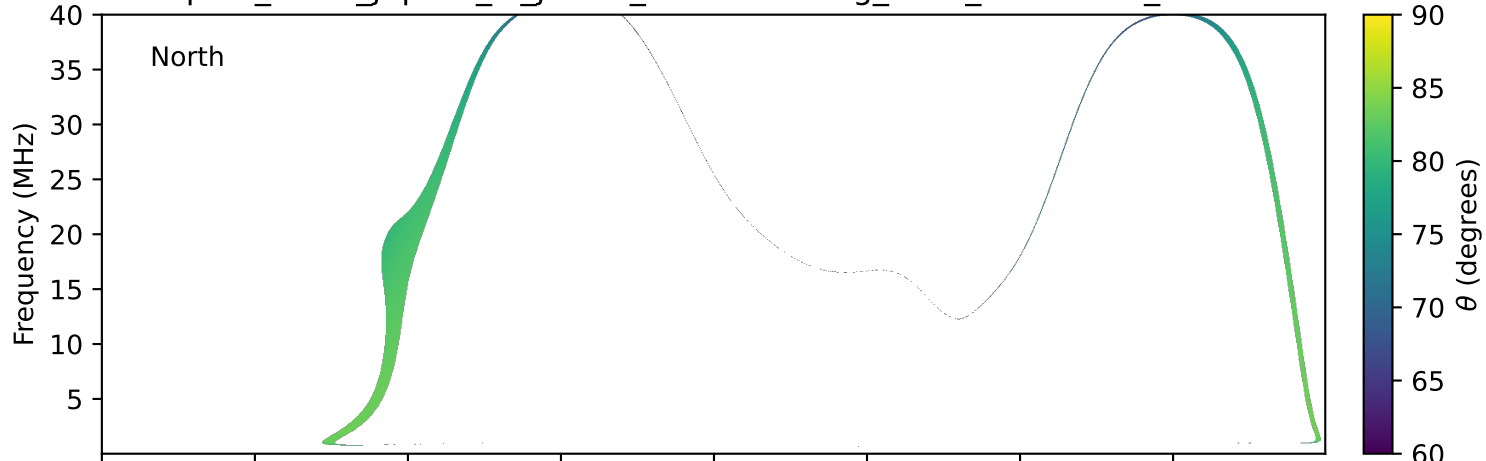
expres_earth_jupiter_io_jrm33_lossc-wid1deg_3kev_19960818_v11.cdf
