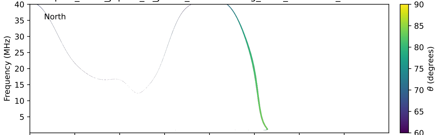
expres_earth_jupiter_io_jrm33_lossc-wid1deg_3kev_19960813_v11.cdf
