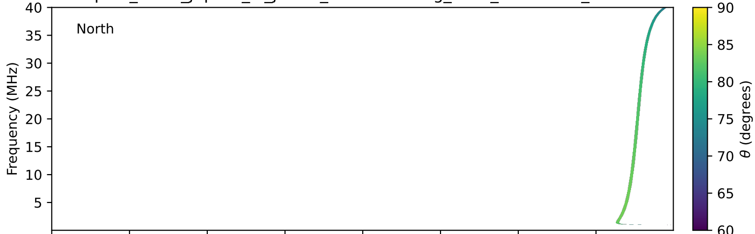
expres_earth_jupiter_io_jrm33_lossc-wid1deg_3kev_19960812_v11.cdf
