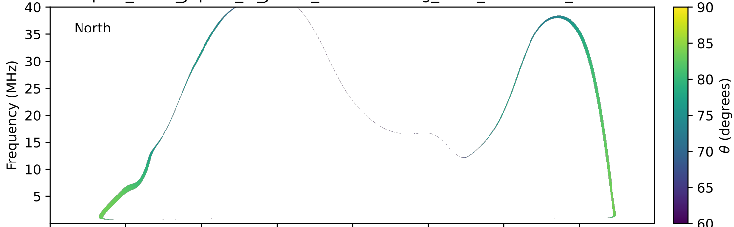
expres_earth_jupiter_io_jrm33_lossc-wid1deg_3kev_19960811_v11.cdf
